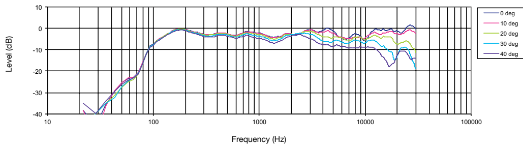
Off-axis Frequency Response
